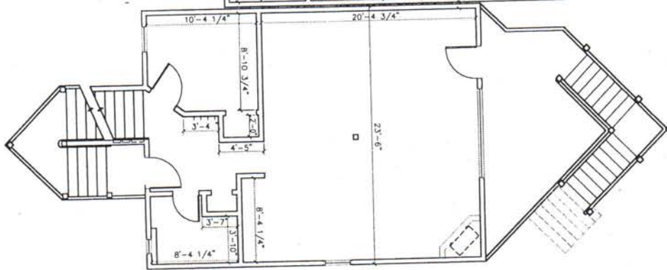
2 UNIT 2, 1ST LEVEL FLOOR PLAN AS-BUILT
